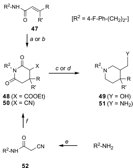
Scheme 2. Reagents and conditions: (a) diethyl malonate, NaOEt, toluene, reflux, 75%; (b) ethyl cyanoacetate, NaH, THF, reflux (45–75%); or KOBut, t -BuOH, THF, reflux (75–96%); (c) LiAlH 4 , THF, reflux (40%); (d) BH 3 , THF, reflux, then HOAc (30–60%); (e) ethyl cyanoacetate, neat, 100 °C, 52%; (f) ethyl β-methylpropenoate, KOBut, t -BuOH, THF, reflux, 85%.
